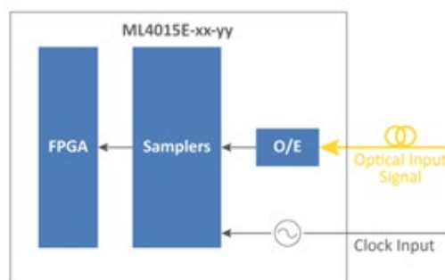
Figure 2: Schematics of the ML4015E-OPT
