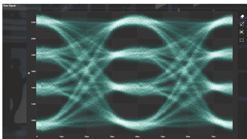
Figure 8: 26.5625 GBaud Optical Eye Diagram – Raw Diagram
