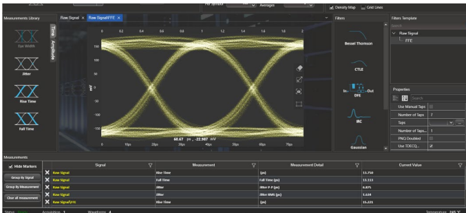
Figure 4: 26.5625 GBaud Optical Eye Diagram
