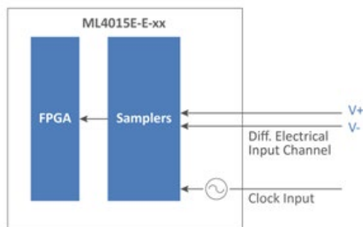
Figure 1: Schematics of the ML4015E-35
